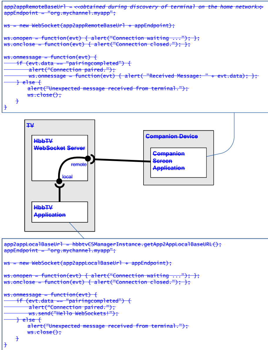
Figure 34: Application to application communication using WebSockets
