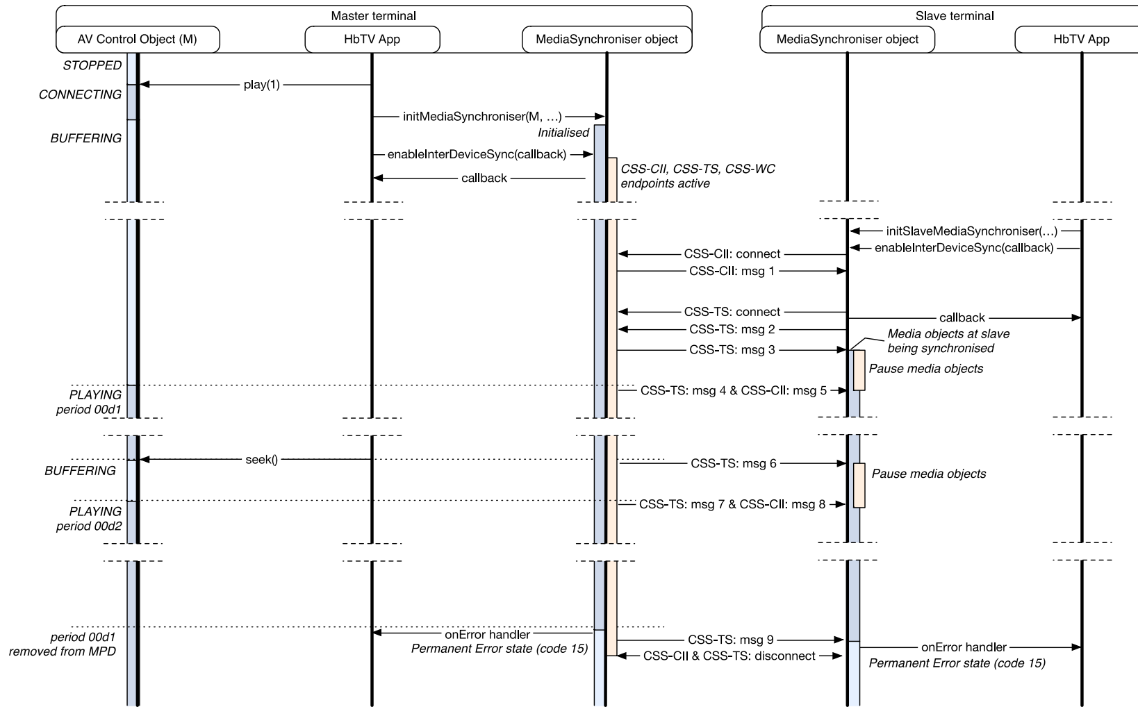
Figure 28: Inter-device synchronization sequence diagram where master media is an AV/V Control object playing an MPEG DASH presentation
