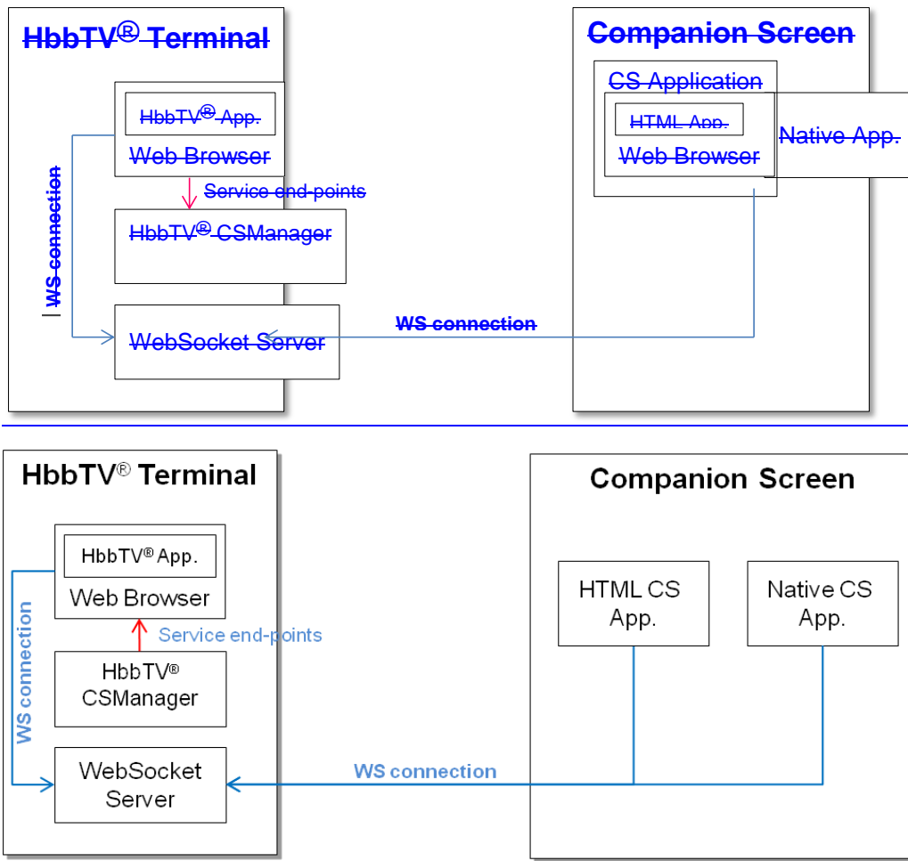
Figure 32: Architecture for application to application communication
