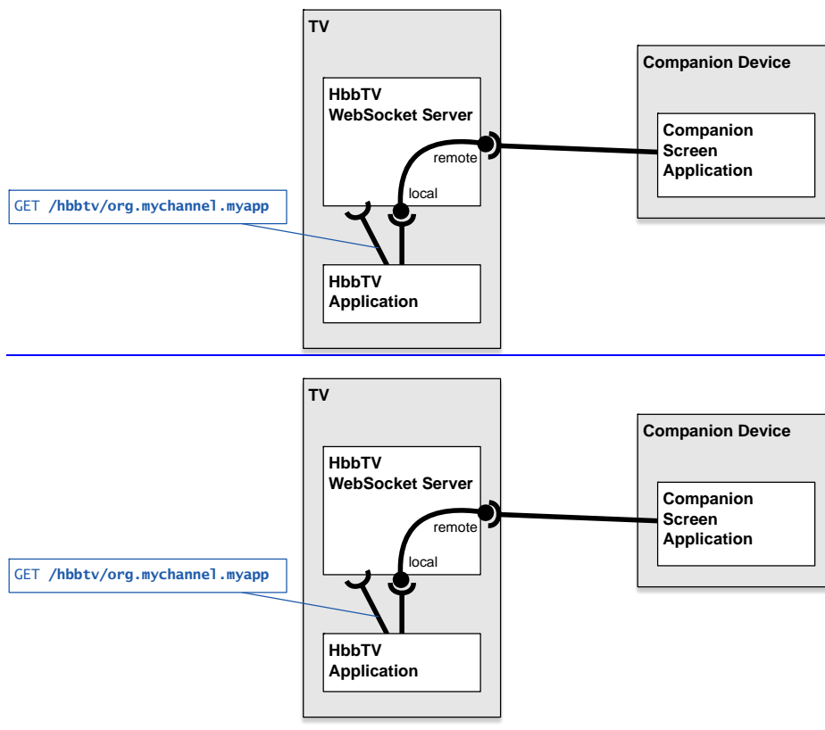
Figure 36: A paired connection for application to application communication
