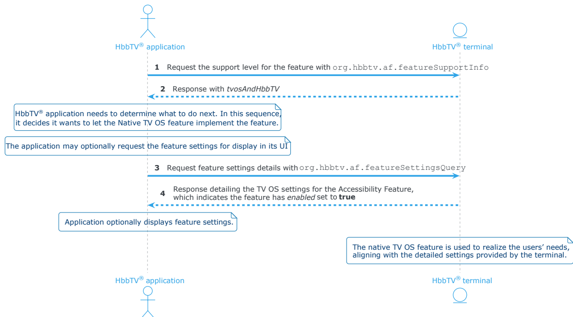
Figure 40: Application lets TV OS be responsible for feature implementation
