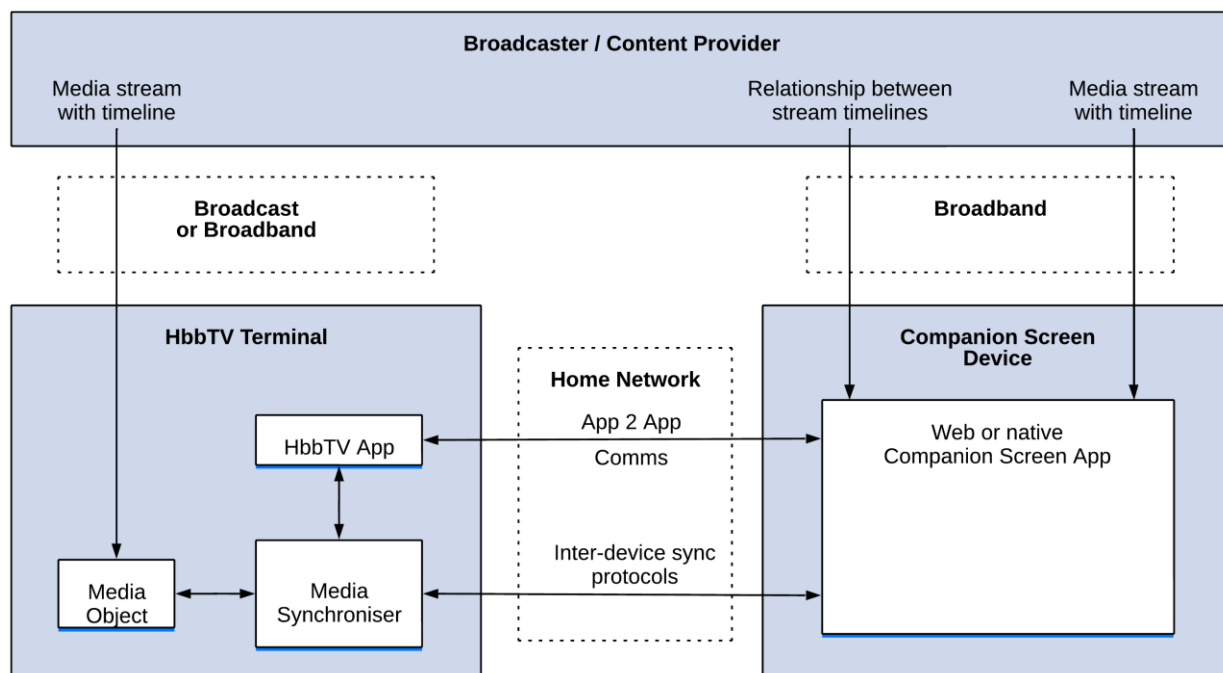
Figure 20: Relationship between MediaSynchroniser object and HbbTV® application for inter-device synchronisation with a CSA
