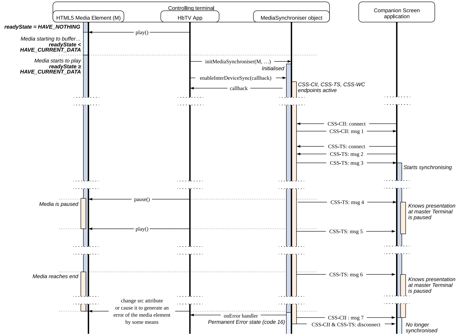
Figure 29: Inter-device synchronisation sequence diagram where synchronisation media is an HTML5 media element playing an MPEG DASH presentation
