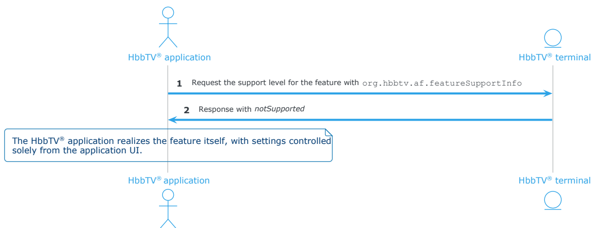
Figure 42: The feature is not supported by the TV
