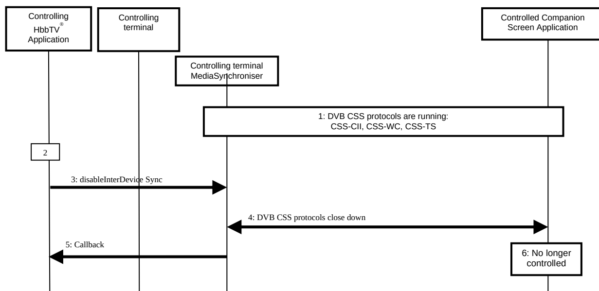
Figure 27: Termination of inter-device timeline synchronisation
