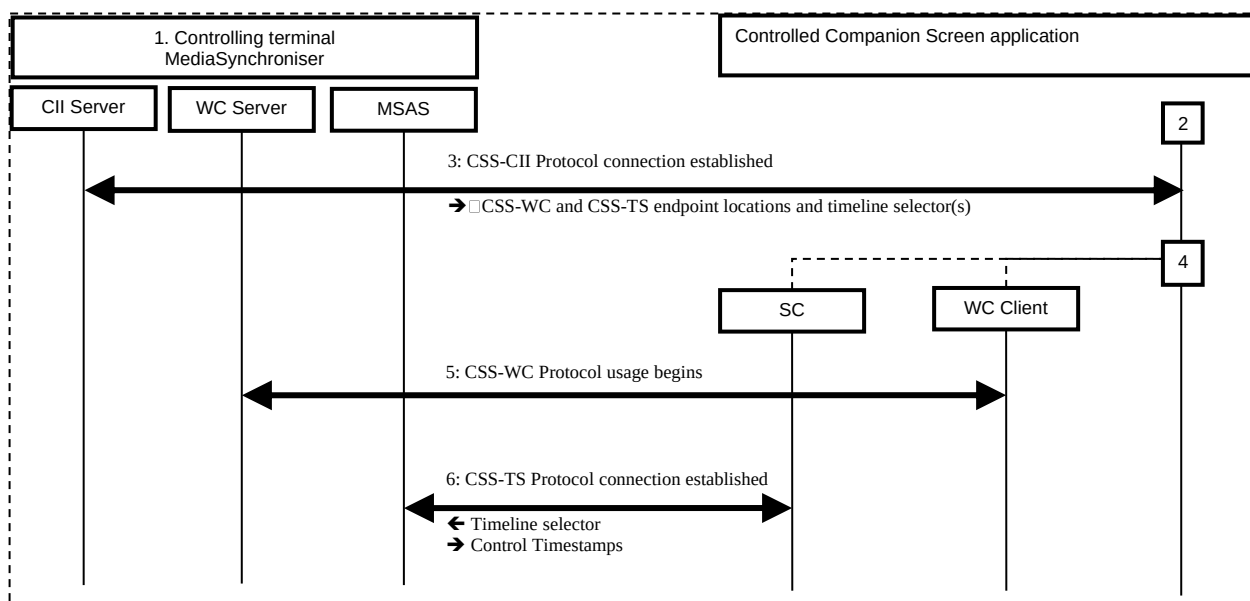
Figure 26: Protocol interactions for inter-device timeline synchronisation
