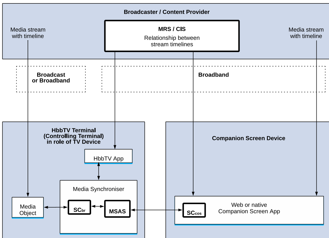
Figure 22: Basic mapping of media synchronisation architecture for inter-device synchronisation
