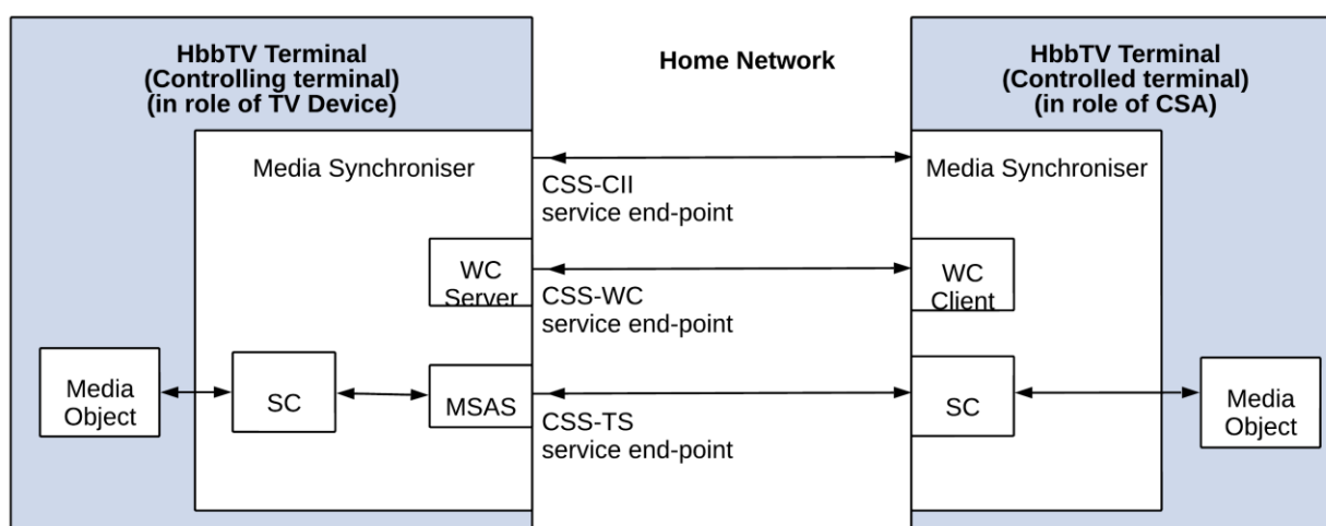
Figure 23: Relationship between the HbbTV ® MediaSynchroniser and MSAS, SC, WC Server and WC Client elementary functions and protocol service endpoints
