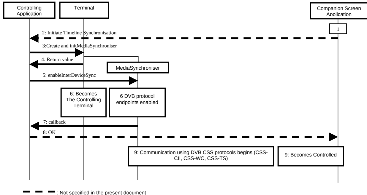
Figure 25: Initiation of inter-device timeline synchronisation
