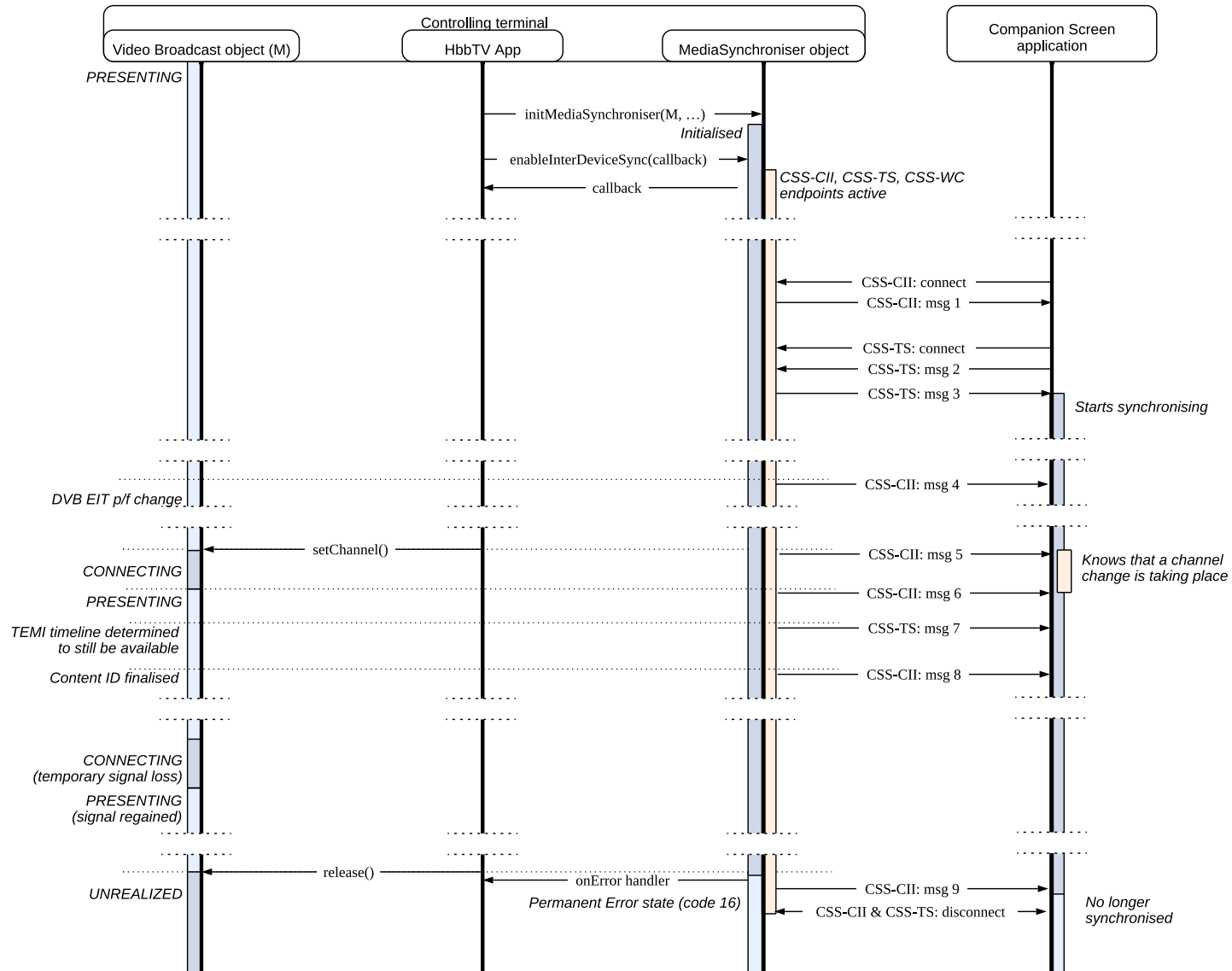
Figure 30: Inter-device synchronisation sequence diagram where synchronisation media is a video/broadcast object
