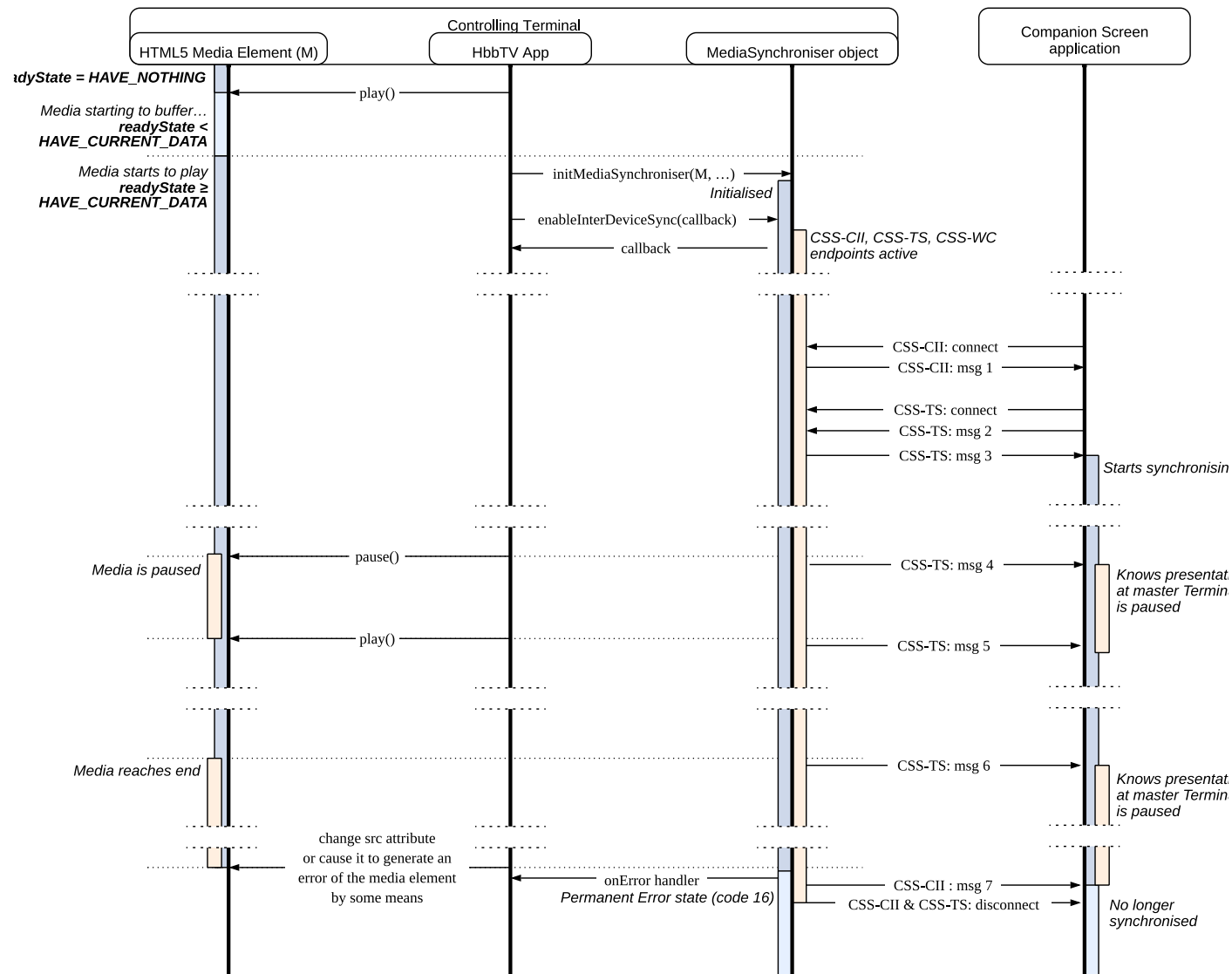
Figure 28: Inter-device synchronisation sequence diagram where the synchronisation media is an HTML5 media element playing ISOBMFF media
