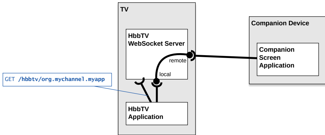
Figure 37: A paired connection for application to application communication
