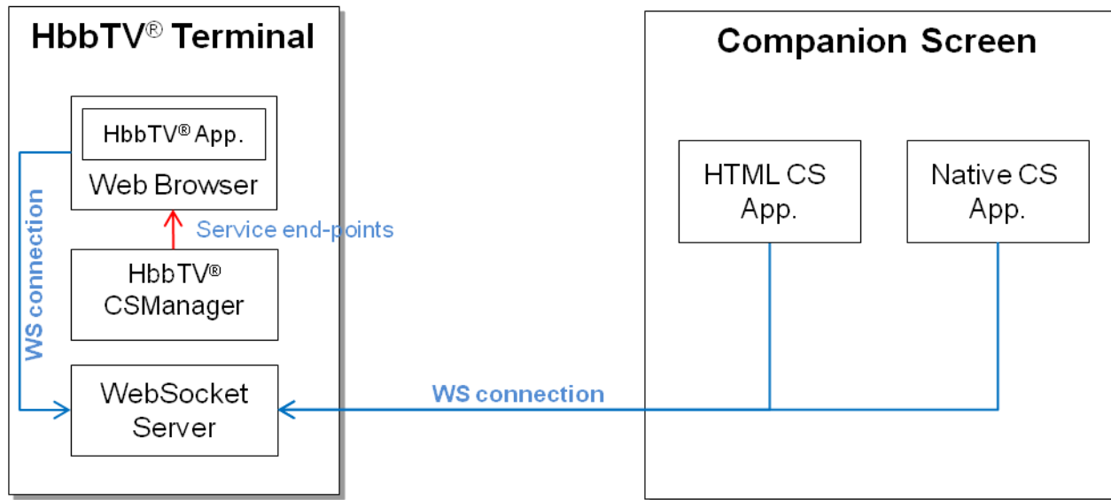
Figure 33: Architecture for application to application communication
