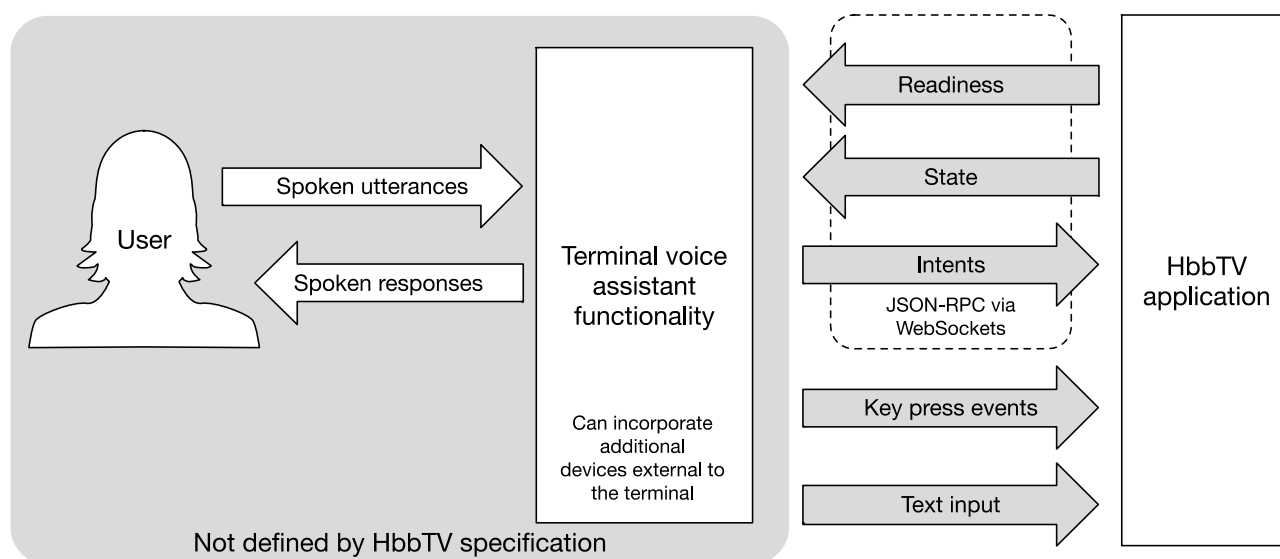
Figure 44: Architecture for voice interaction
