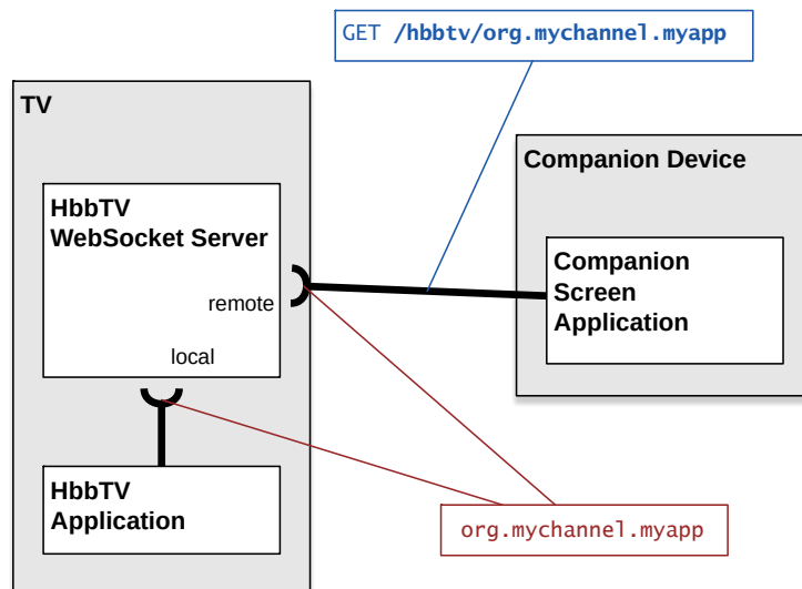
Figure 38: Two waiting connections that will be paired by the TV
