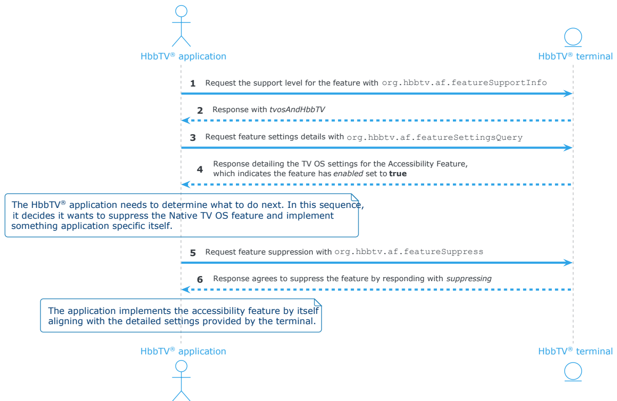
Figure 39: Application requests suppression of a TV OS native feature
