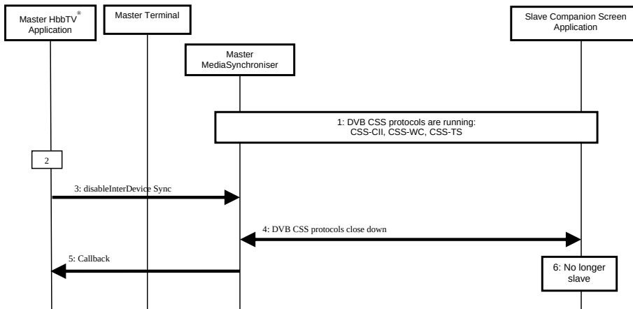
Figure 29: Termination of inter-device timeline synchronization
