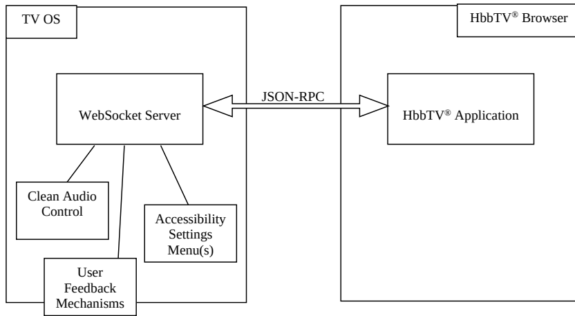
Figure 40a: Overview of the Accessibility Support Framework
