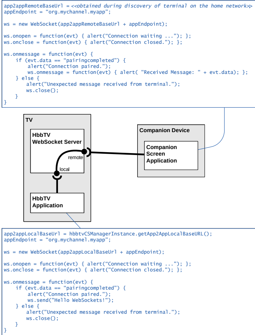
Figure 37: Application to application communication using WebSockets
