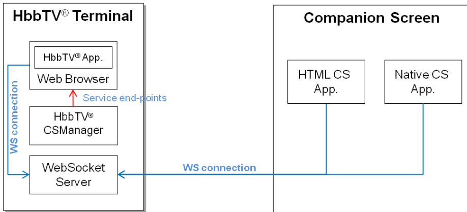
Figure 35: Architecture for application to application communication
