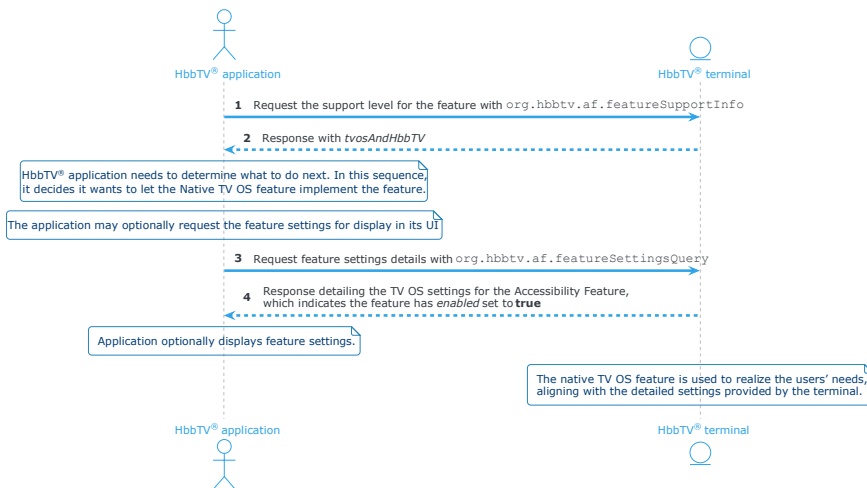
Figure 42: Application lets TV OS be responsible for feature implementation
