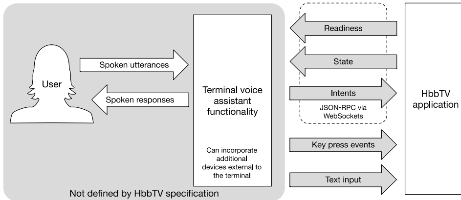
Figure 46: Architecture for voice interaction
