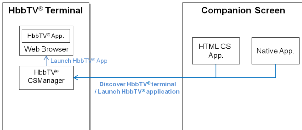
Figure 36: Architecture for remotely launching HbbTV® applications
