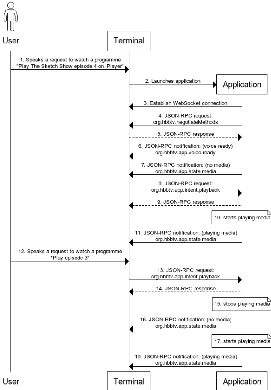
Figure P.5: Voice interaction example - initiating playback
