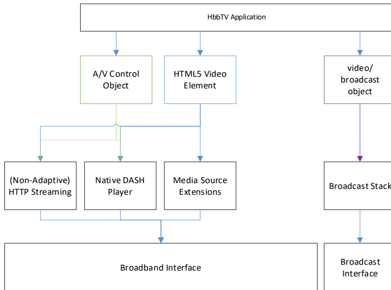
Figure O.1: Media APIs - Minimal
