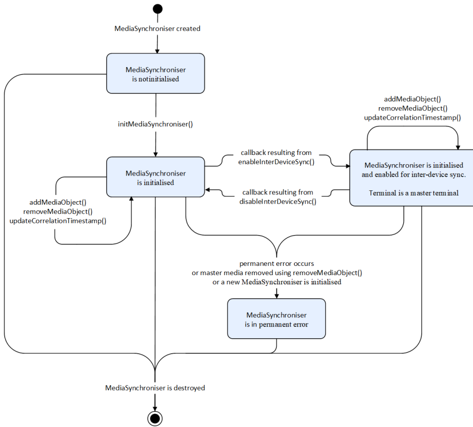
Figure 26: Media Synchronization states
