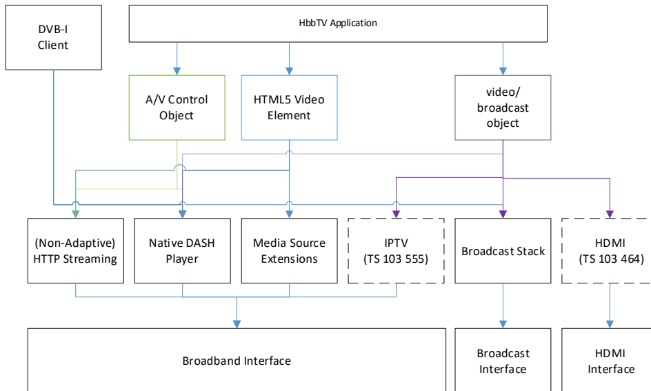
Figure O.2: Media APIs - Complete
