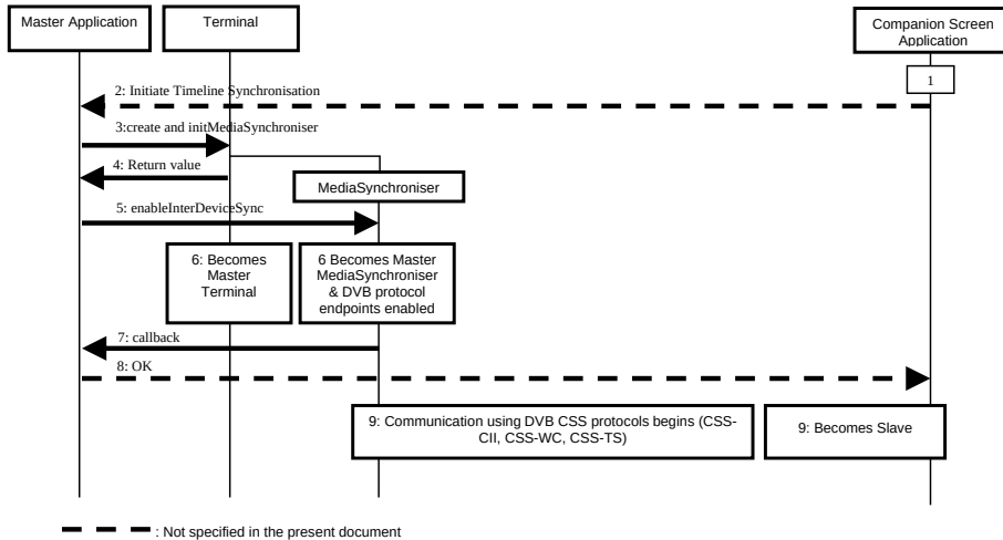
Figure 27: Initiation of inter-device timeline synchronization
