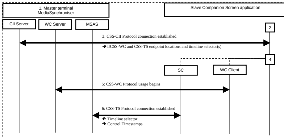
Figure 28: Protocol interactions for inter-device timeline synchronization
